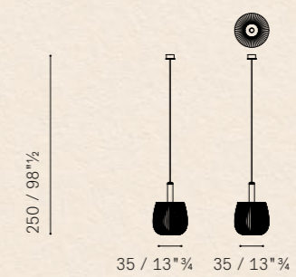
Soffi — Chandelier no. 18 medium lamps
